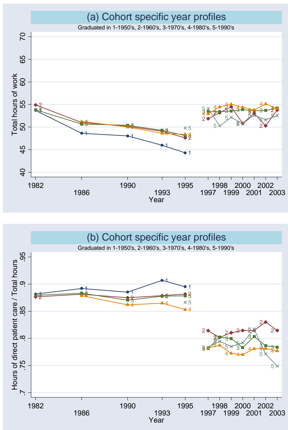
Figure 5. Total hours of work: Male GP/FPs, by Year
