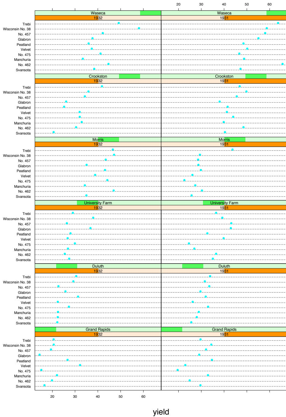
Figure 10.7: Default strip labels for categorical conditioning variables.
