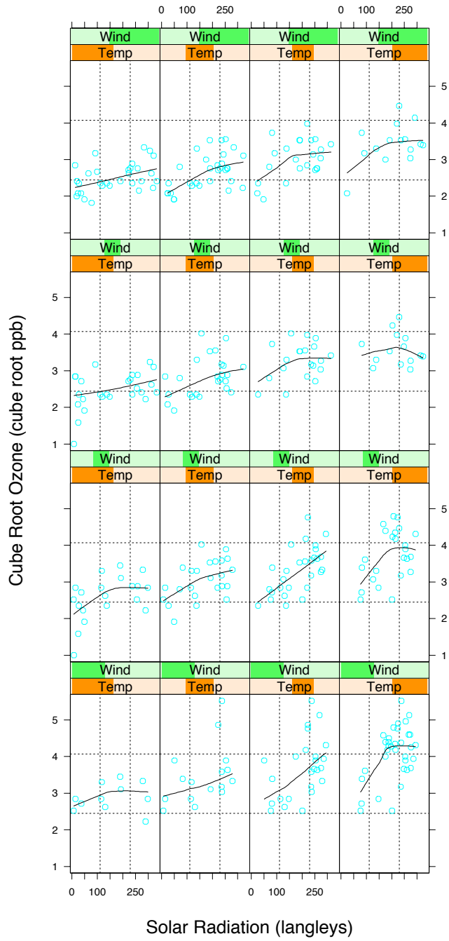
Figure 18.4: Scatterplot with grids and loess curves.
